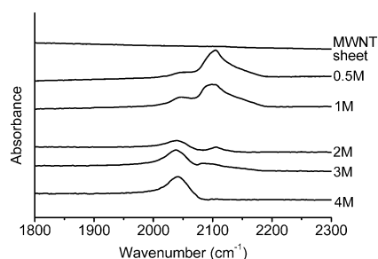
Figure 8. FTIR spectra in the 1800\text{--}2300\text{ cm}^{-1} region for polynitrogen-MWNT sheets after electrochemical synthesis with different azide concentrations. MWNT background has been subtracted for the polynitrogen-MWNT curves.
